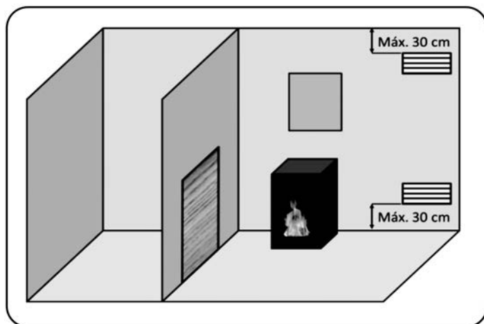
Indicative diagram for ventilation grilles.
